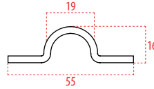
U Kanal Ray (Çift Rulmanlı Makaralara Uygun) U Channel Track (suitable for 2 bearing wheels)
