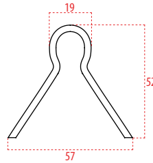
R Kanal Ray R Channel Track (cement fixing)
